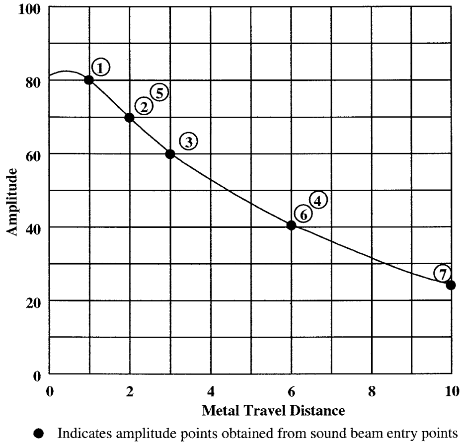
FIG. A1.4 Typical Angle Beam Standardization at 45° for Flat Surfaces of Thick Specimens
