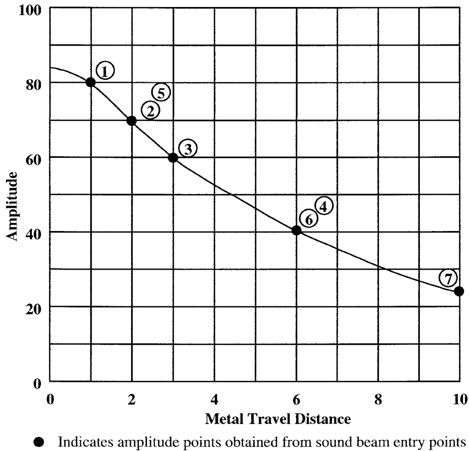
FIG. A1.3 Typical Angle Beam Standardization at 60° for Flat Surfaces of Thin Specimens
